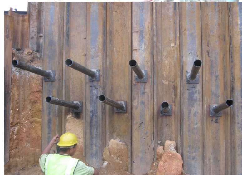
Project : The Construction & Completion of Facilities Works (Package A) For The Kelana Jaya (KJL) Line Extension - Sheet Piling with T-System Nailing
