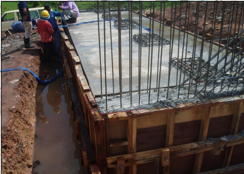
Project : Kolej Pertanian Malaysia (KPM), Bukit Tangga, Kedah Darul Aman - Bridge Structure Works
